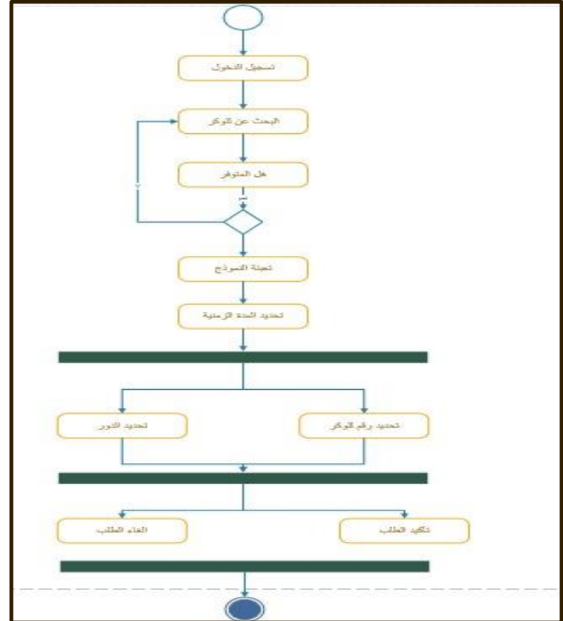
Activity Diagram
